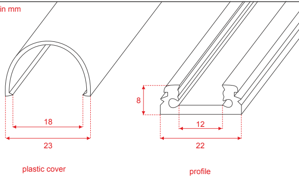
A9930020 Alu profile 22 Aluminum profile for round covercap
